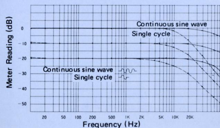
Peak Level Meter Response
