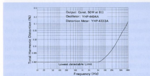
Output Power vs. Total Harmonic Distortion
