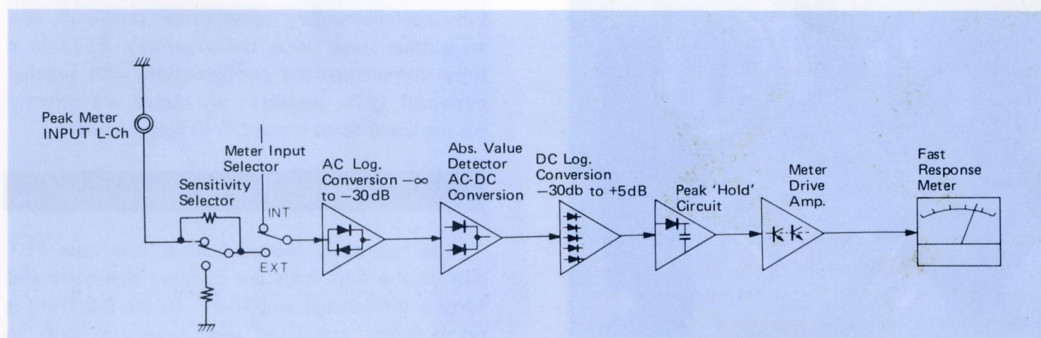
Meter Circuit Block Diagram
