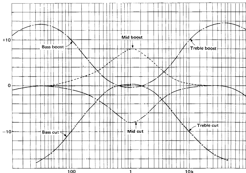
Figure 16-2 TONE CONTROL CHARACTERISTIC
