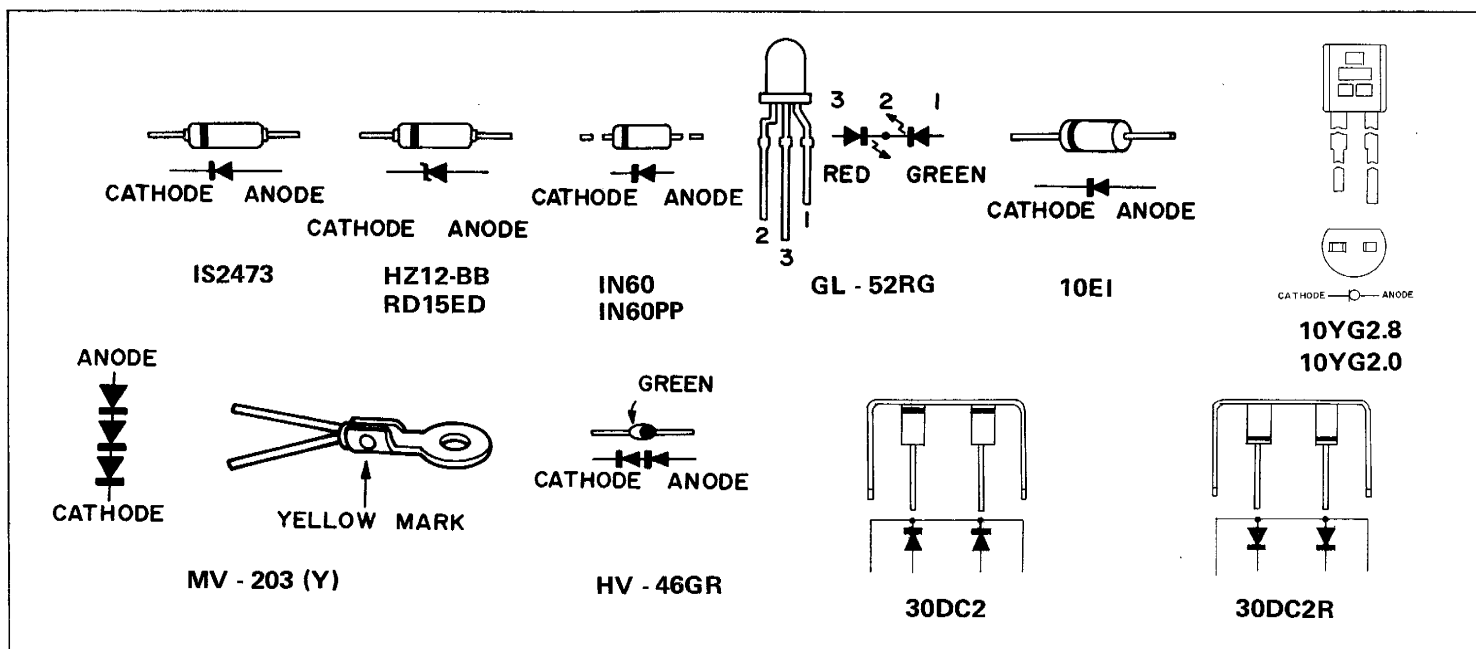
Figure 33-1 DIODE TYPES
