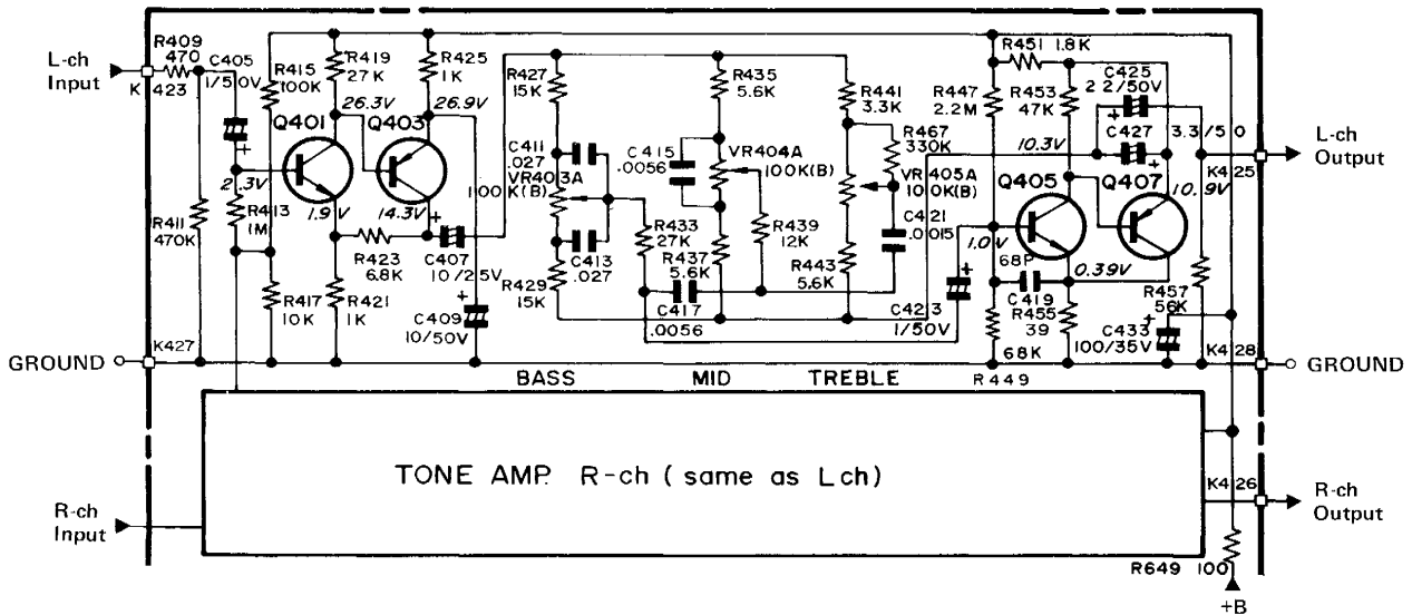
Figure 16-1 TONE CONTROL CIRCUIT
