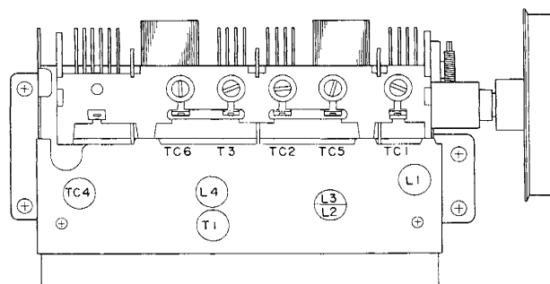
Figure 25 ALIGNMENT POINTS OF RF/IF P.W. BOARD
